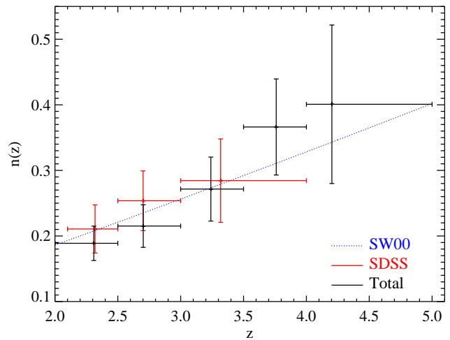
FIG. 3.— Incidence of damped Ly \alpha systems per unit redshift n(z) as a function of redshift for the SDSS-DR1 (red points) and total samples (black points). The vertical error bars reflect 1\sigma uncertainty assuming Poissonian statistics and the horizontal bars indicate the redshift interval. The dotted blue line is the fit to n(z) from Storrie-Lombardi and Wolfe (2000): n(z) = 0.055(1+z)^{1.11} .
